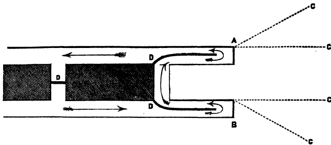
Fig. 197. The Pillar and Stall System. A, B. Main working-places. C, C, C, C. Exploring bore-holes. D, D, D. Brattices, or timber partitions to confine the air (shown by the arrows) in its proper channel, and make it sweep round the place where the men are working at A, B. The shaded parts represent the pillar left to support the roof.
